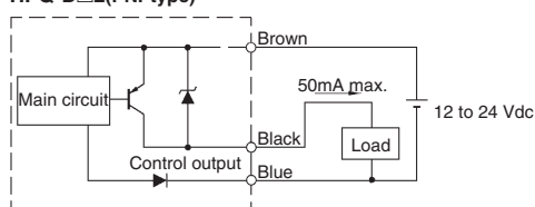
HPQ-D□2(PNPtype)
