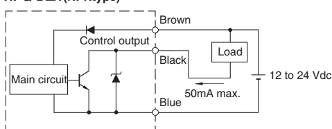
HPQ-D□1(NPNtype)
